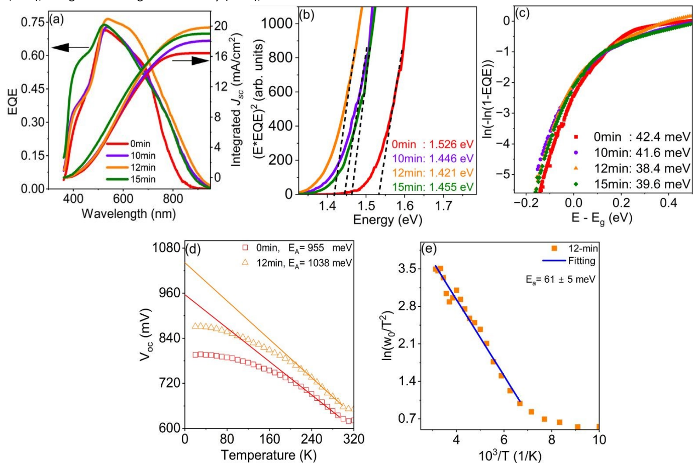
Figure 8. (a) External quantum efficiency (EQE) spectra and integrated J_{sc} from EQE of CZTS solar cells subjected to post-annealing for various durations (SC2-0 min, SC2-10 min, SC2-12 min, and SC2-15 min) and (b) extracted bandgaps ( E_g^* ) of the corresponding absorber layers. (c) Urbach energy ( E_U ) plots derived from EQE data, indicating sub-bandgap tail states. (d) Temperature dependent V_{oc} curves for SC2-0 min and SC2-12 min devices, used to determine activation energy ( E_A ) from the extrapolated y-axis intercept at T = 0 K. (e) Thermal admittance spectroscopy of the SC2-12 min device, revealing defect state energetics.
