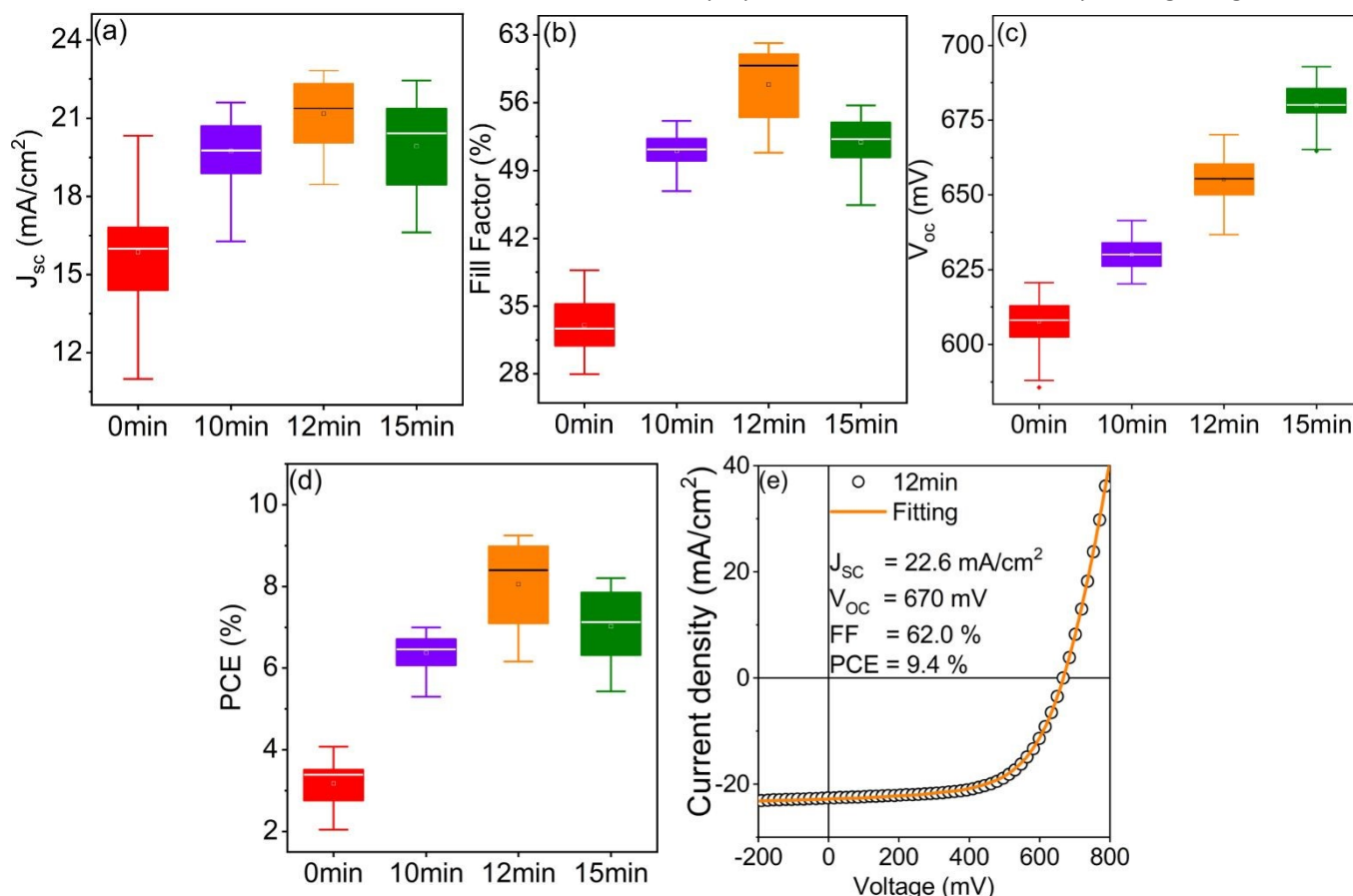
Figure 7. Plots of solar cell output parameters: (a) J_{sc} , (b) FF, (c) V_{oc} , and (d) PCE for SC2 device subjected to different post-annealing durations of the complete Glass/Mo/CZTS/CdS/i-ZnO/ITO structure (SC2-0min, SC2-10min, SC2-12min, and SC2-15min); (e) J-V curve of the champion device with corresponding fitting result using Equation 16.
