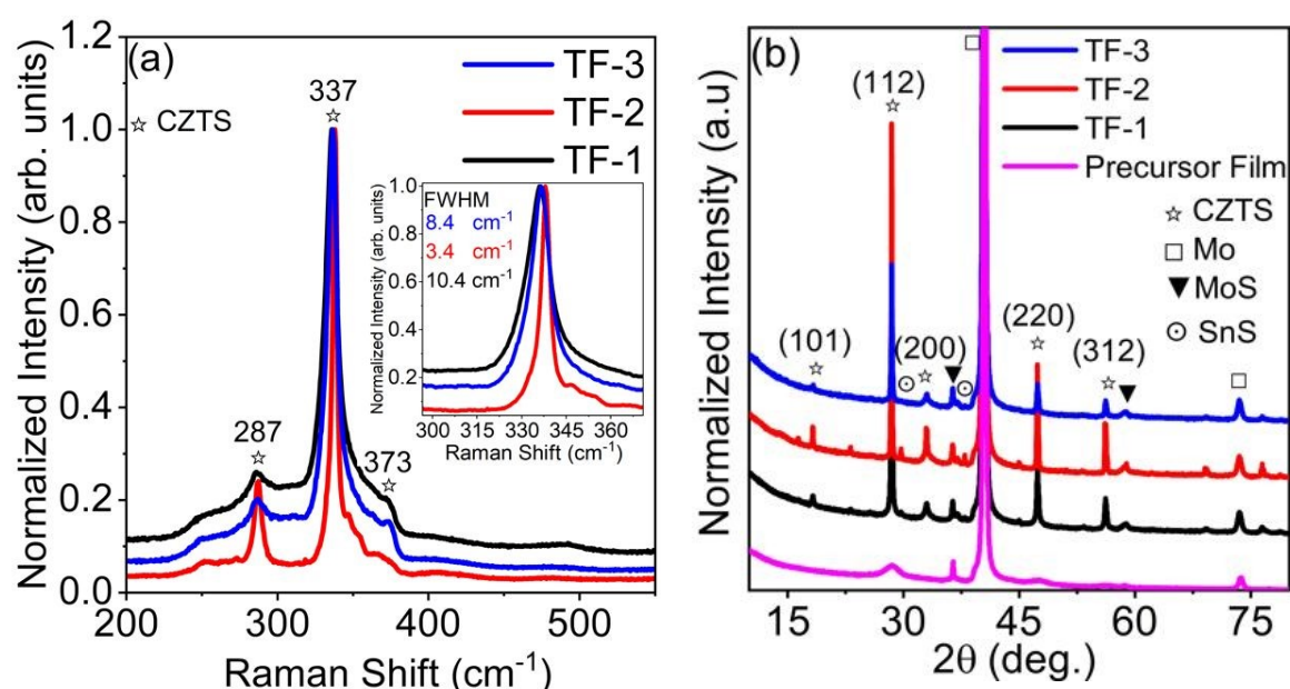
Figure 5. (a) Raman spectra of CZTS thin films (TF) after sulfurization, corresponding to TF-1, TF-2, and TF-3. (b) XRD patterns of CZTS thin films (TF) from different solutions: TF-1, TF-2, and TF-3. The sulfurization process was conducted at 650°C for 20 minutes.
