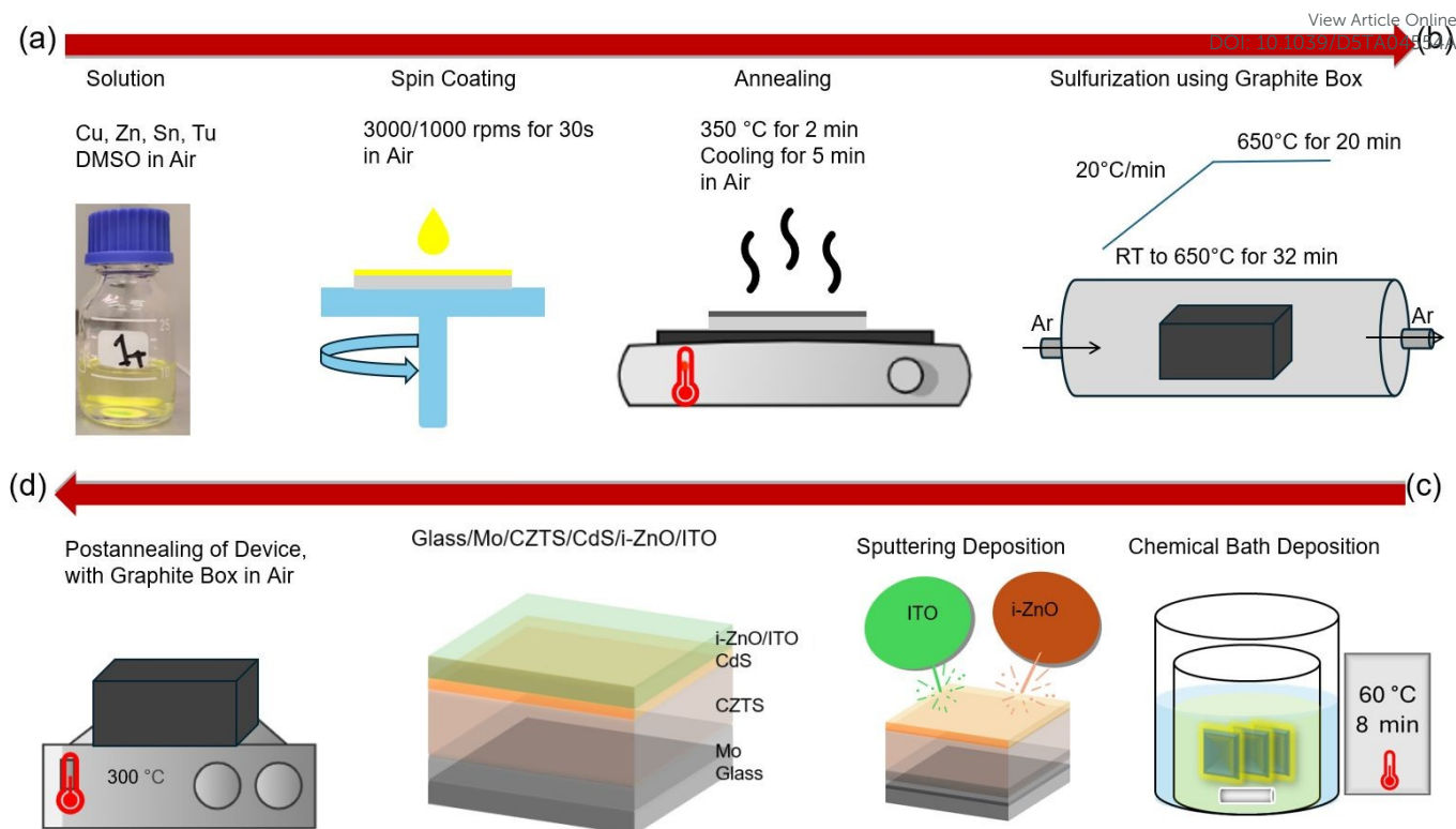
Figure 1. Schematic illustration of the fabrication process for solution-processed CZTS solar cells. (a–b) Preparation of CZTS absorber layer: the precursor solution was formulated in DMSO, followed by spin coating, brief annealing on a hotplate, and high-temperature sulfurization in a graphite box using a tube furnace. (c–d) Device fabrication steps: chemical bath deposition (CBD) of CdS buffer layer, RF sputtering of intrinsic ZnO and ITO as window layers, and post-annealing of the device on a hotplate inside a graphite enclosure under ambient conditions.
