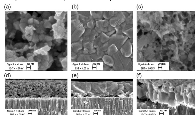
Figure 4. Top-view (a) TF-1, (b) TF-2, and (c) TF-3, and cross-sectional view (d) TF-1, (e) TF-2, and (f) TF-3, SEM images of the CZTS thin film (TF) annealed at 650°C for 20 min.
