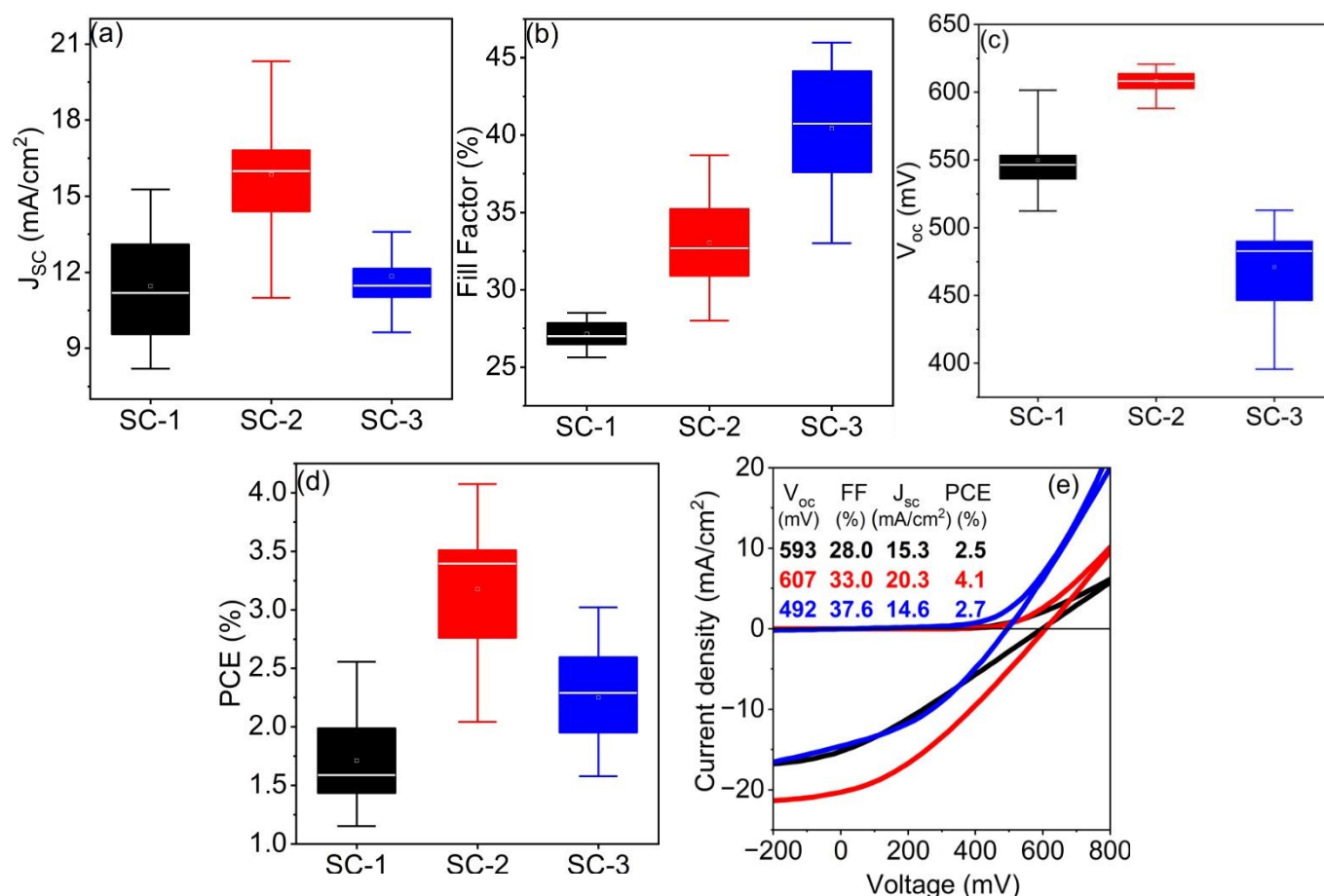
Figure 6. Box plots of the SC-1, SC-2, and SC-3 devices before post-annealing illustrate the statistical distributions of solar cell parameters: (a) Short-Circuit Current Density ( J_{sc} ), (b) Fill Factor (FF), (c) Open-Circuit Voltage ( V_{oc} ), and (d) Power conversion efficiency (PCE). (e) Current–voltage ( J – V ) curves extracted from the highest cell efficiency of SC-1, SC-2, and SC-3 under AM 1.5 illumination ( 100 \text{ mW cm}^{-2} ), with corresponding V_{oc} , FF, J_{sc} , and PCE values.
