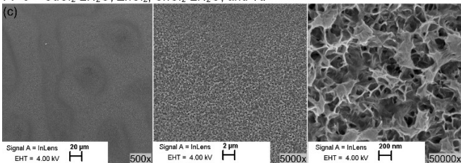
Figure 2. Top-view SEM images of CZTS precursor films (PF): (a) PF-1, (b) PF-2, and (c) PF-3, each shown at magnifications of 500x, 5000x, and 50000x. All precursor films were air-annealed at 350°C for 2 minutes and cooled for 5 minutes, with the cycle repeated eight times.
