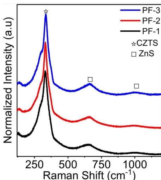
Figure 3. Raman spectra of CZTS precursor film (PF) before sulfurization, prepared from different solutions: PF-1, PF-2, and PF-3.
